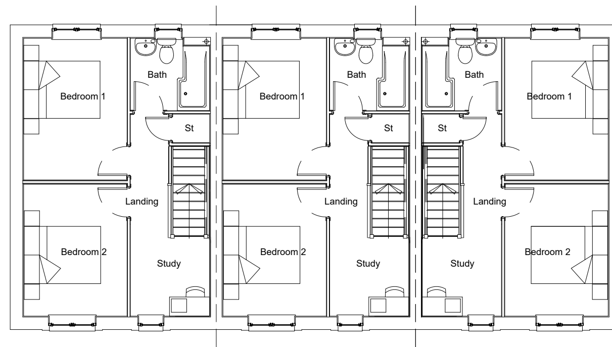
First Floor
